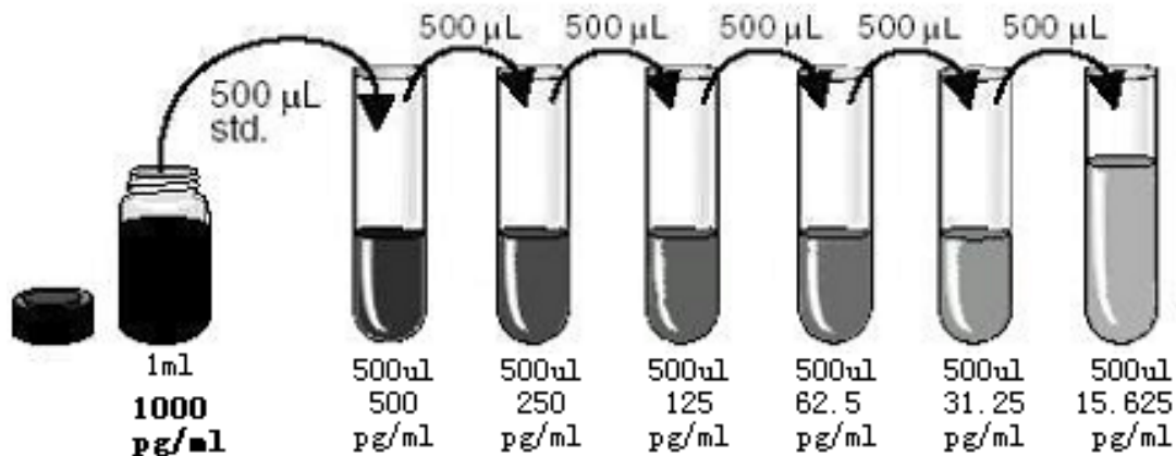
Figure 1 : Preparation of IL-15 standard dilutions
