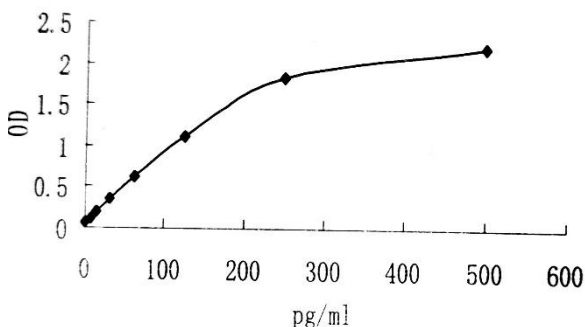
Figure 3: Representative standard curve for TSLP ELISA. TSLP was diluted in serial two-fold steps in Sample Diluent.
