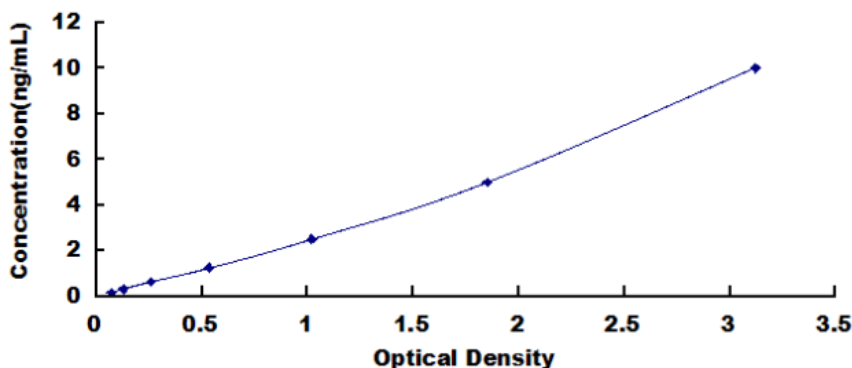
Typical Standard Curve for Rabbit ANXA5 ELISA.
