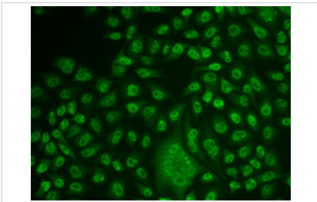
Immunofluorescence analysis of U2OS cells using TFPT .
