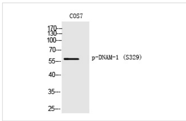
Western Blot analysis of COS7 cells using Phospho-DNAM-1 (S329) Polyclonal Antibody
