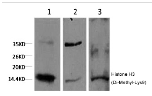
Western blot analysis of 1) HeLa, 2) Rat Heart Tissue, 3) Raw264.7, diluted at 1:2000.
