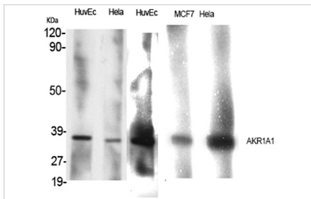
Western Blot analysis of HELA HuvEc MCF7 cells using AKR1A1 Polyclonal Antibody
