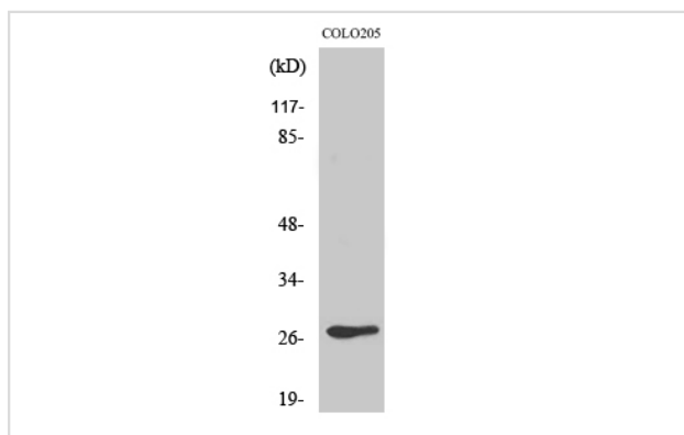
Western Blot analysis of MCF7 cells using Olfactory receptor 5D3 Polyclonal Antibody
