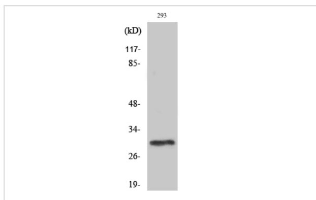
Western Blot analysis of Jurkat cells using PIG-X Polyclonal Antibody
