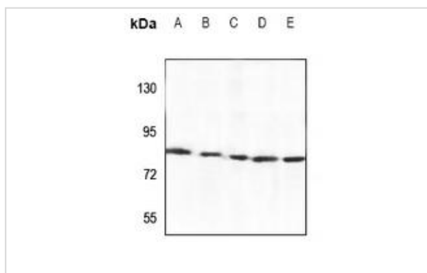
Western blot analysis of TBX3 expression in CT26 (A), MEF (B), C6 (C), HEK293T (D), HepG2 (E) whole cell lysates
