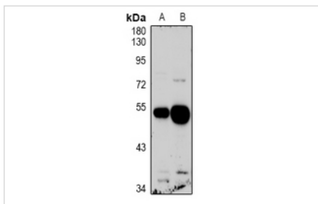
Western blot analysis of GPR103 expression in U87MG (A), HEK293T (B) whole cell lysates.
