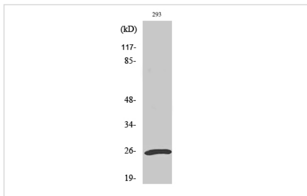
Western Blot analysis of 293 cells using UCH-L1 Polyclonal Antibody
