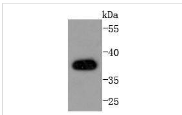
Western blot analysis of AMPK beta 1 on A431 cells lysates using anti-AMPK beta 1 antibody at 1/1,000 dilution.
