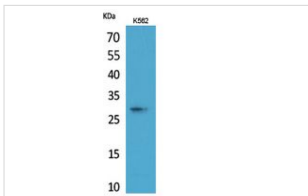
Western Blot analysis of K562 cells using ApoA-I Polyclonal Antibody.
