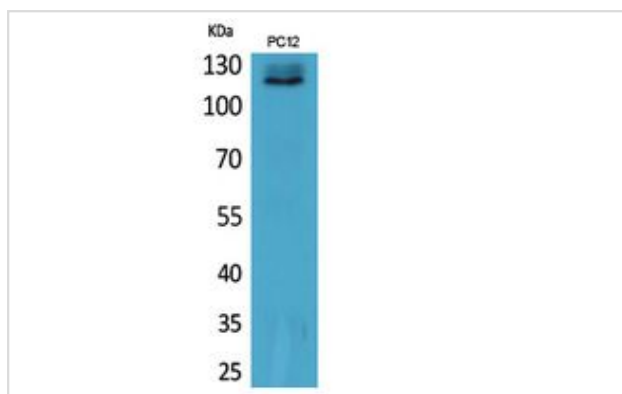
Western Blot analysis of PC12 cells using UBA1 Polyclonal Antibody.
