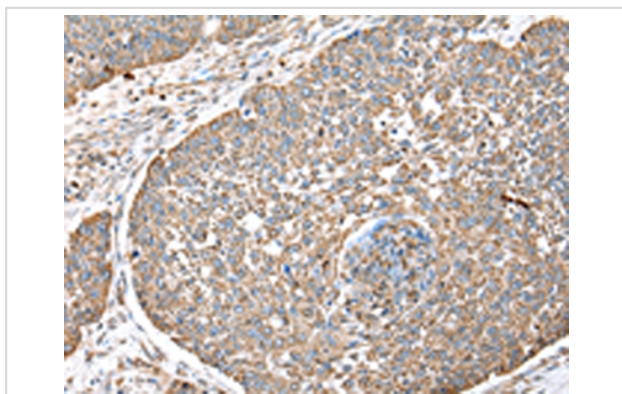
Immunohistochemical analysis of paraffin-embedded Human lung cancer tissue using #42855 at dilution 1/40.
