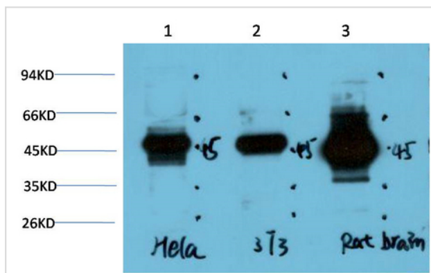
Western blot analysis of 1) Hela Cell Lysate, 2) 3T3 Cell Lysate, 3) Rat Brain Tissue Lysate using GSK3 \beta Mouse mAb diluted at 1:1000.
