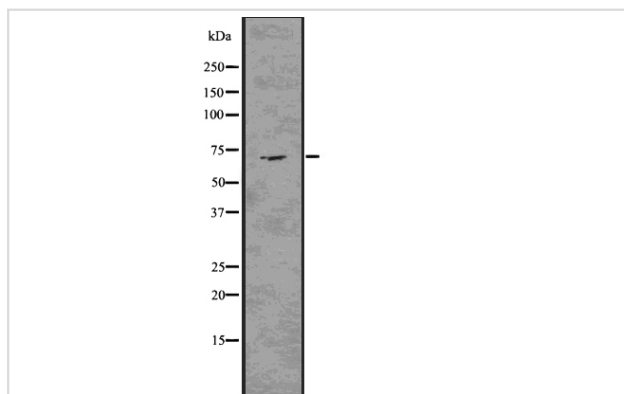
Western blot analysis Elastin using HepG2 whole cell lysates
