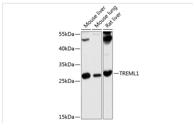
Western blot analysis of extracts of various cell lines, using TREML1 at 1:1000 dilution.
