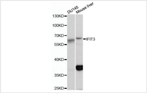
Western blot analysis of extracts of various cell lines, using IFIT3 at 1:1000 dilution.
