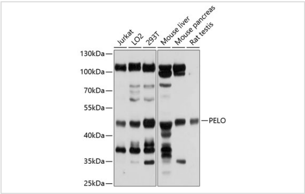
Western blot analysis of extracts of various cell lines, using PELO at 1:1000 dilution.
