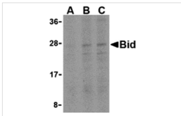
Western blot analysis of Bid in A549 cell lysates with Bid antibody at (A) 0.5, (B) 1, and (C) 2 ug/mL.
