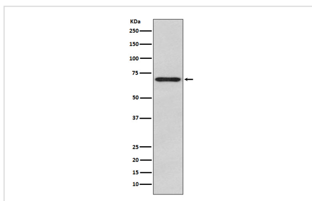
Western blot analysis of Glypican 3 expression in HepG2 cell lysate.
