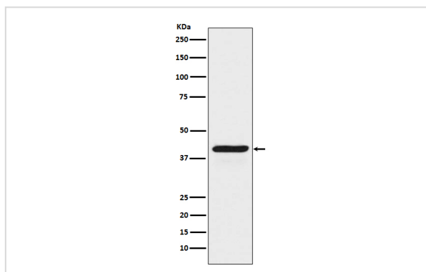
Western blot analysis of INDO expression in HeLa cell lysate treated with IFN gamma.
