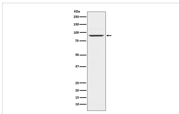
Western blot analysis of Prolactin Receptor expression in Jurkat cell lysate.
