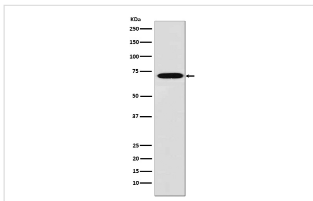
Western blot analysis of Plastin L expression in THP1 cell lysate.
