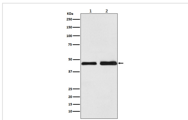
Western blot analysis of Oxytocin Receptor expression in (1) Jurkat cell lysate; (2) Mouse spleen lysate.
