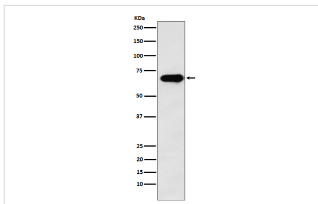
Western blot analysis of SAM68 expression in A431 cell lysate.
