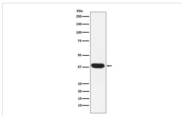
Western blot analysis of MYF5 expression in Human skeletal muscle lysate.
