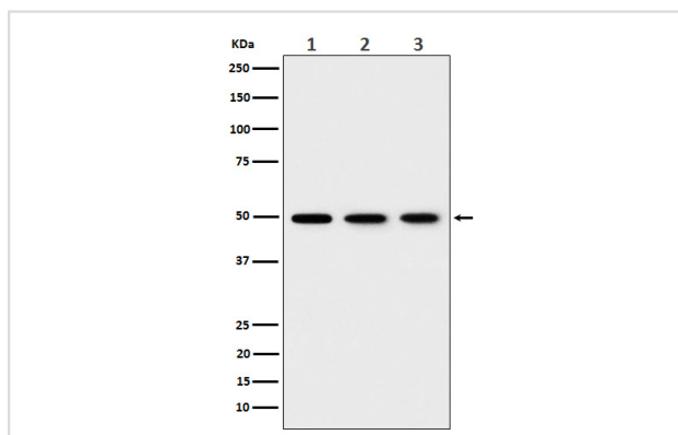
Western blot analysis of EEF1G expression in (1) 293T cell lysate; (2) HepG2 cell lysate; (3) NIH/ 3T3 cell lysate.
