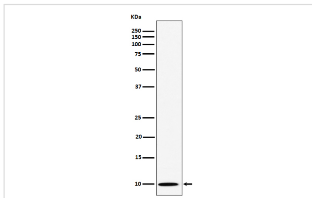
Western blot analysis of NOP10 expression in Jurkat cell lysate.
