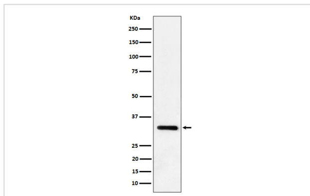
Western blot analysis of IL-33 expression in mouse lung cell lysate.
