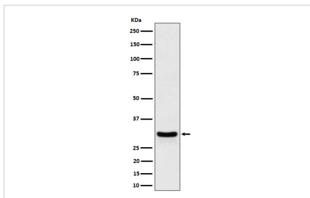
Western blot analysis of FRAT1 expression in HeLa cell lysate.
