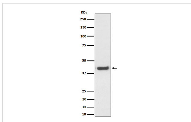
Western blot analysis of MVK expression in HepG2 cell lysate.
