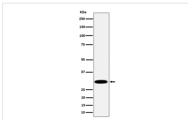
Western blot analysis of TPMT expression in Jurkat cell lysate.
