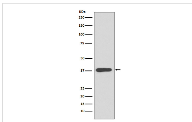
Western blot analysis of MBP expression in E.coli lysate.
