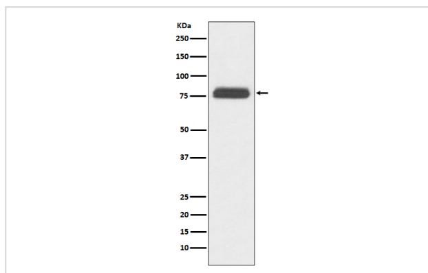
Western blot analysis of TBR1 expression in human fetal brain lysate.
