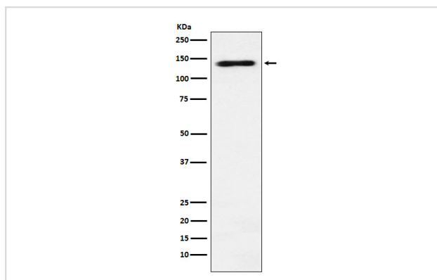
Western blot analysis of RNA Helicase A expression in Jurkat cell lysate.
