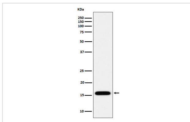
Western blot analysis of MGST1 expression in HepG2 cell lysate.
