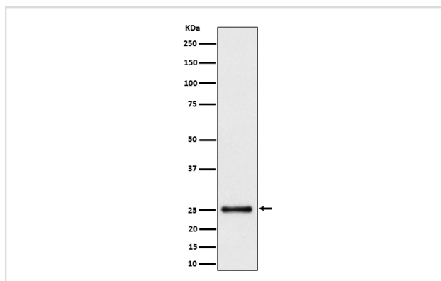
Western blot analysis of HMG4 expression in HeLa cell lysate.
