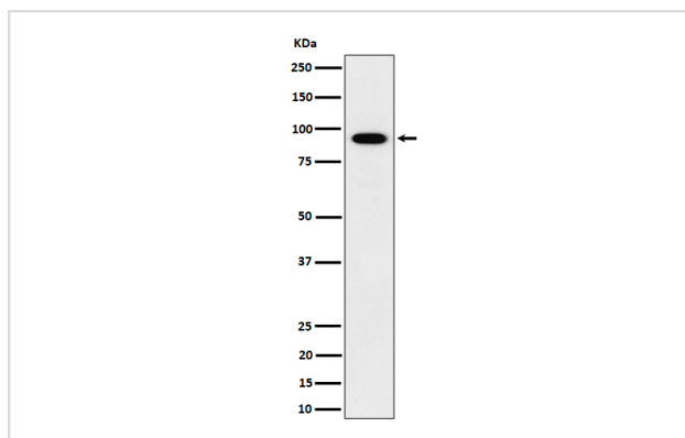
Western blot analysis of IFT88 expression in HepG2 cell lysate.
