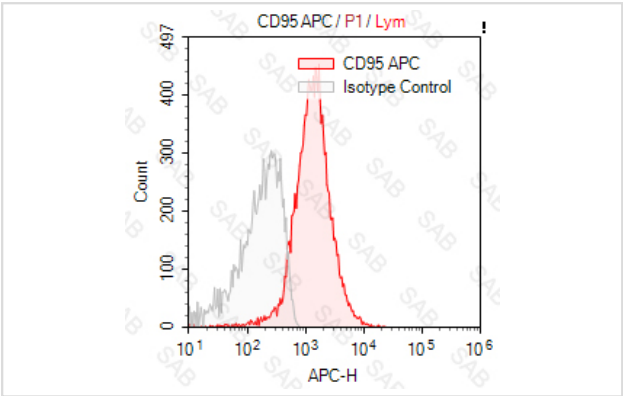
Human peripheral blood lymphocytes stained with APC anti-human CD95 (colored histogram) or APC mouse IgG1 κ (gray histogram)
