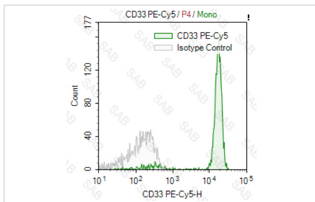
Human peripheral blood monocytes stained with PE-Cy5 anti-human CD33 (colored histogram) or PE-Cy5 mouse IgG1 (gray histogram)
