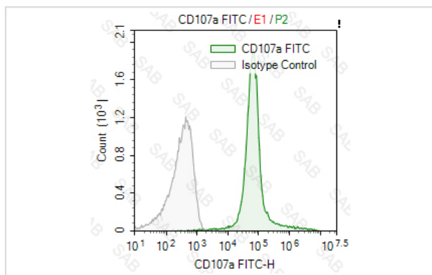
Fixed /permeabilized Jurkat cells stained with FITC anti-human CD107a (colored histogram) or FITC mouse IgG1 κ (gray histogram)
