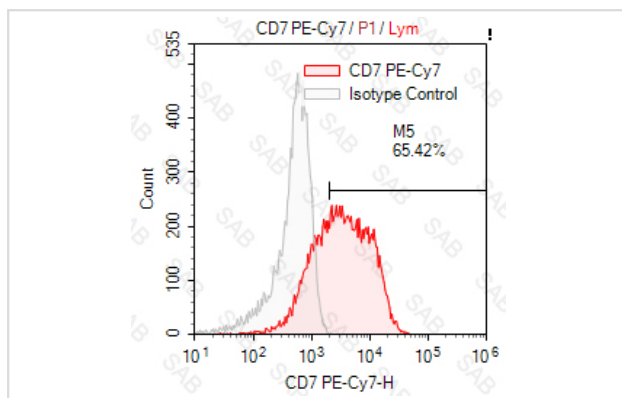
Human peripheral blood lymphocytes stained with PE-Cy7 anti-human CD7 (colored histogram) or PE-Cy7 mouse IgG1 κ (gray histogram)
