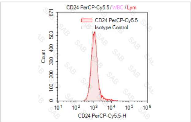
Human peripheral blood lymphocytes stained with PerCP-Cy5.5 anti-human CD24 (colored histogram) or PerCP-Cy5.5 mouse IgG1 (gray histogram)
