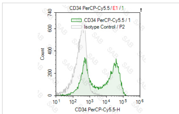
Two mixed TF-1 cells and HEL cells stained with PerCP-Cy5.5 anti-human CD34 (colored histogram) or PerCP-Cy5.5 mouse IgG1 κ (gray histogram)
