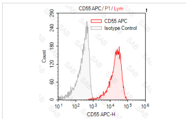
Human peripheral blood lymphocytes stained with APC anti-human CD55 (colored histogram) or APC mouse IgG1 (gray histogram)
