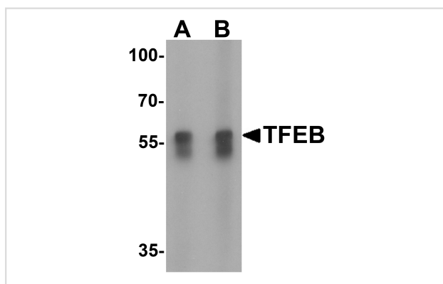
Western blot analysis of TFEB in A549 cell lysate with TFEB antibody at (A) 1 and (B) 2 ug/mL.
