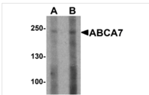
Western blot analysis of ABCA7 in 293 cell lysate with ABCA7 antibody at (A) 1 and (B) 2 ug/ml.
